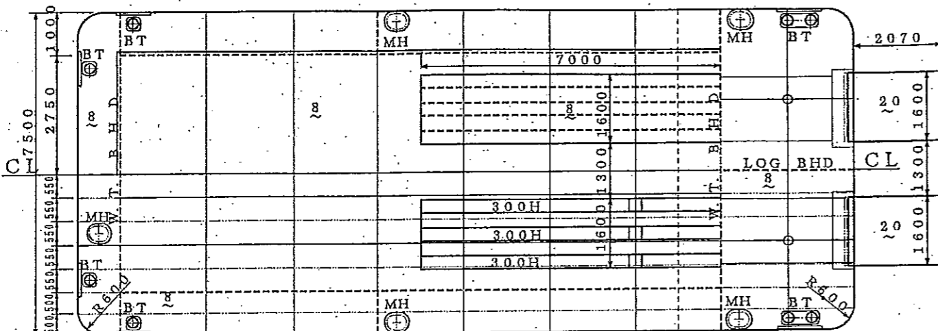
DECK PLAN
