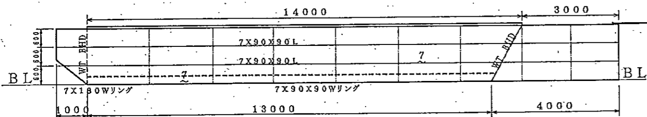
SIDE SECTION
