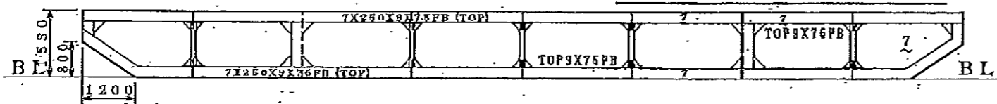
GIRDER SECTION
