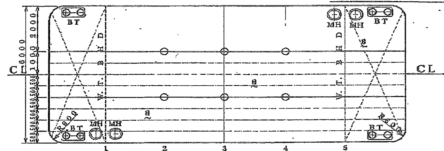
DECK PLAN
