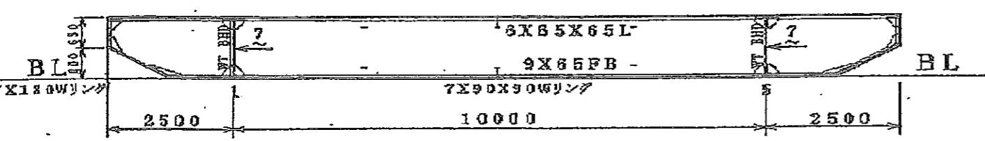
GIRDER SECTION
