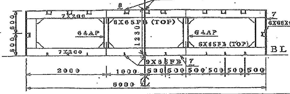
WEB FRAME SECTION 8XB5X65L (FR2. 3. 4)
