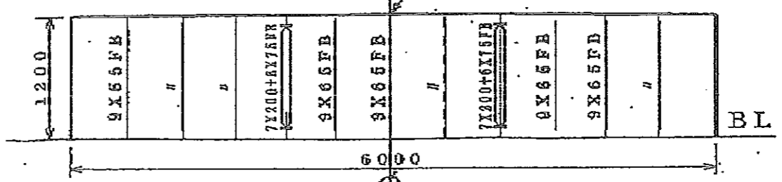
WEB FRAME SECTION 8XB5X65L (FR2. 3. 4)
