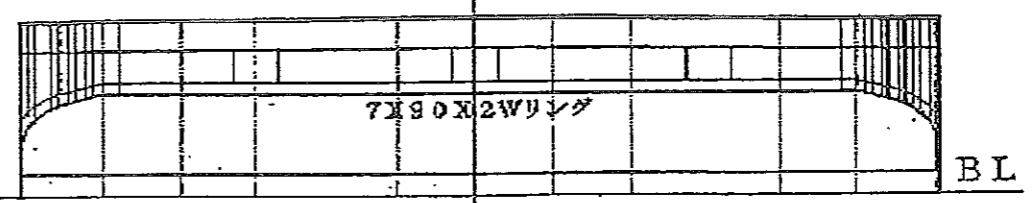
W. T. BHD SECTION CAMBER (FR1. 5)
